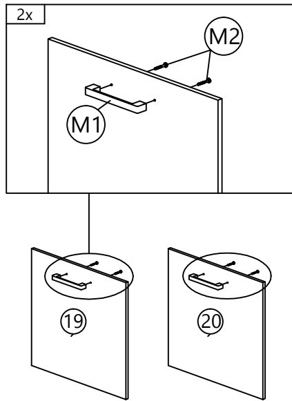
Outside View
